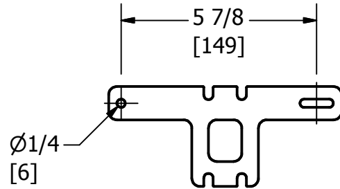
Adapter Bracket
